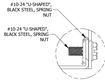
DETAIL A (4 PL.) (LID ATTACHMENT DETAIL)
