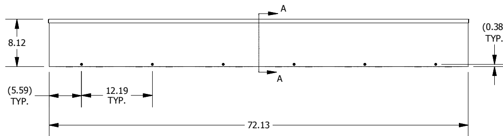
FRONT VIEW
