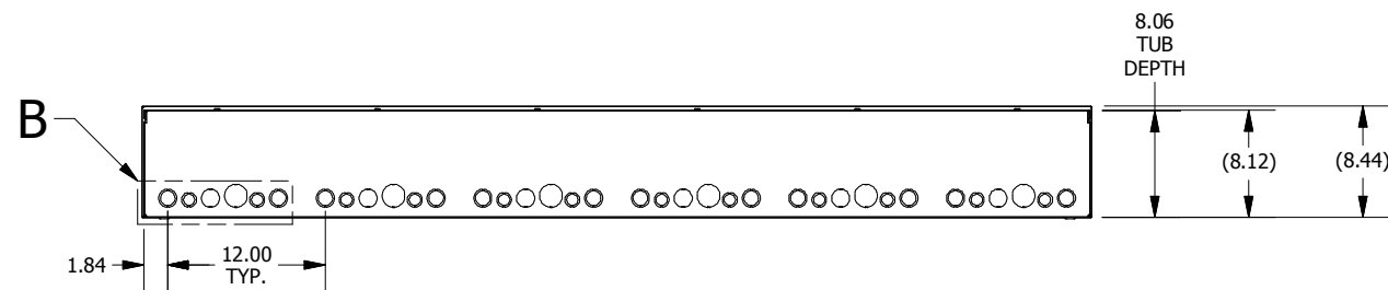
BOTTOM VIEW
