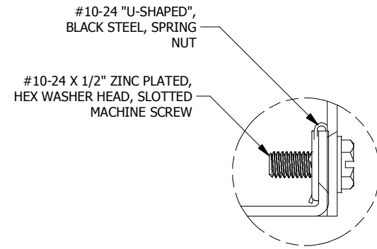
DETAIL A (3 PL.) (LID ATTACHMENT DETAIL)
