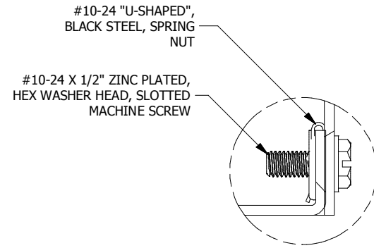
DETAIL A (6 PL.) (LID ATTACHMENT DETAIL)
