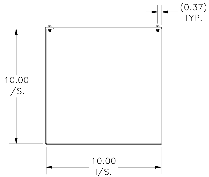
RIGHT VIEW
