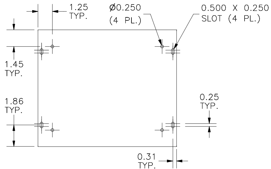
BOTTOM VIEW
