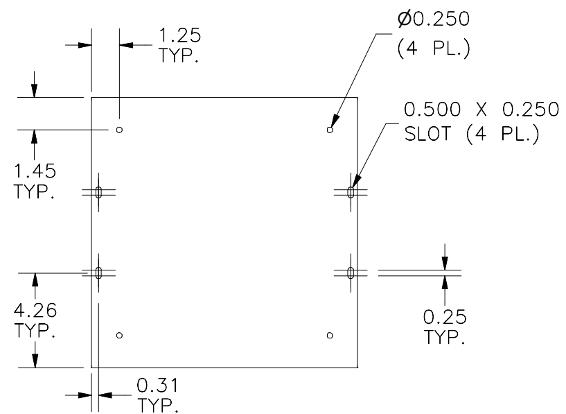
BOTTOM VIEW
