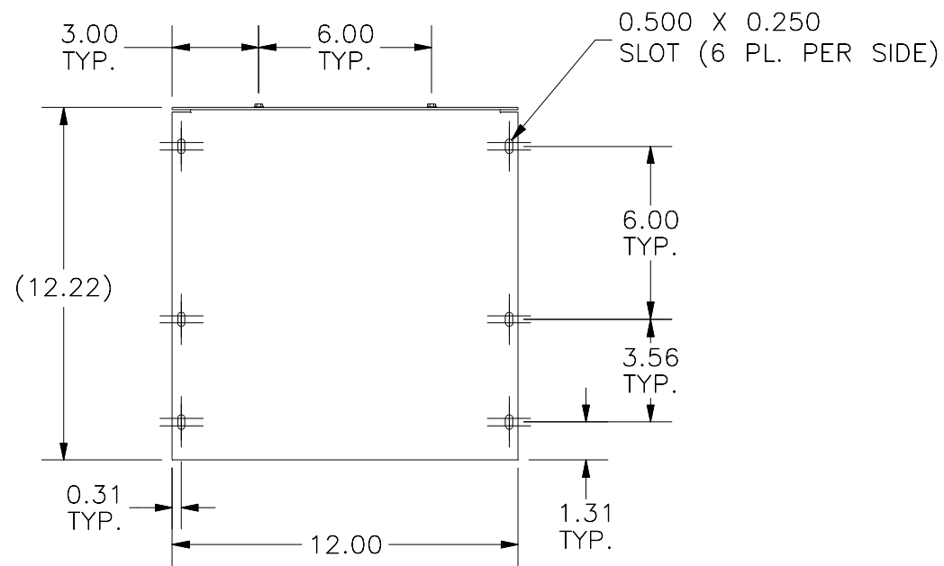
FRONT VIEW
