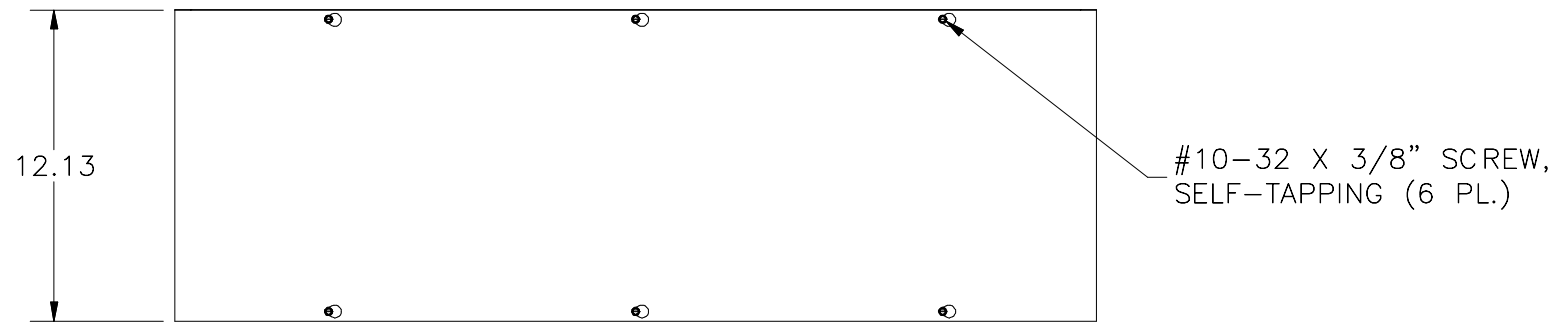
TOP VIEW
