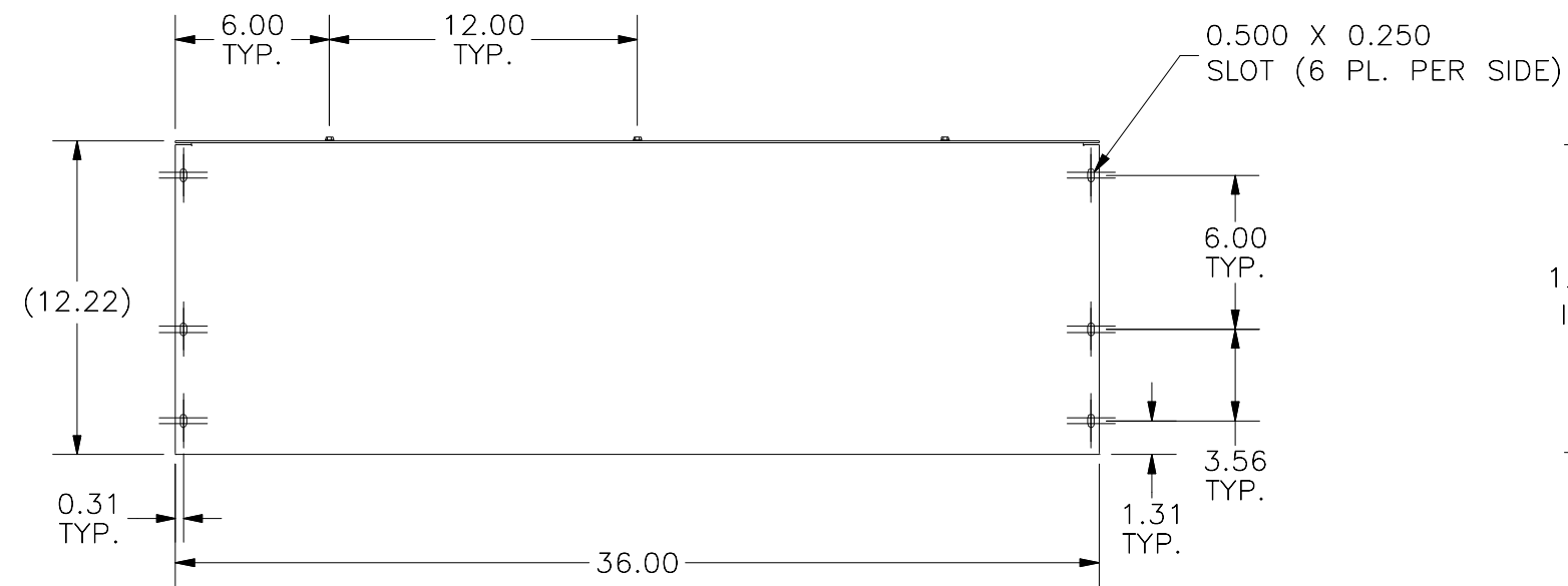
FRONT VIEW
