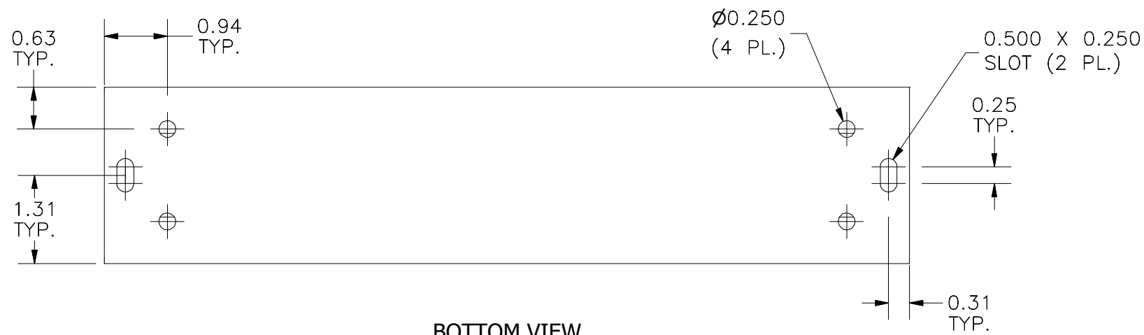
BOTTOM VIEW
