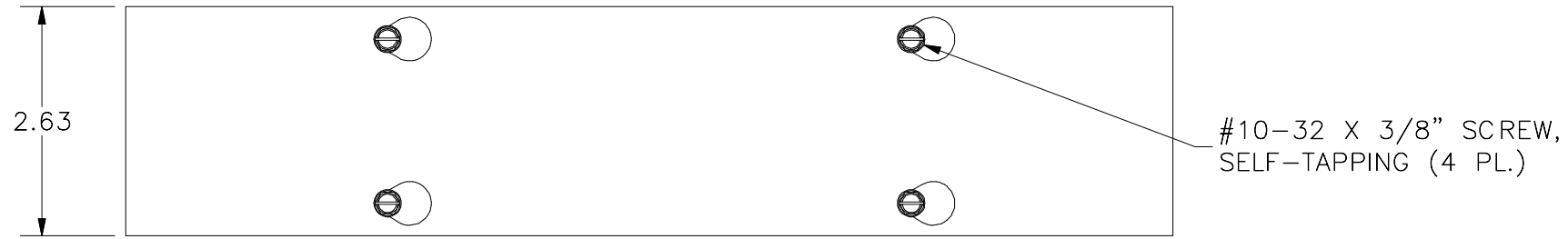
TOP VIEW
