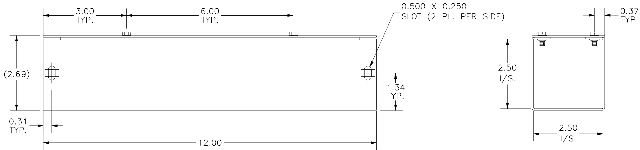
FRONT VIEW
