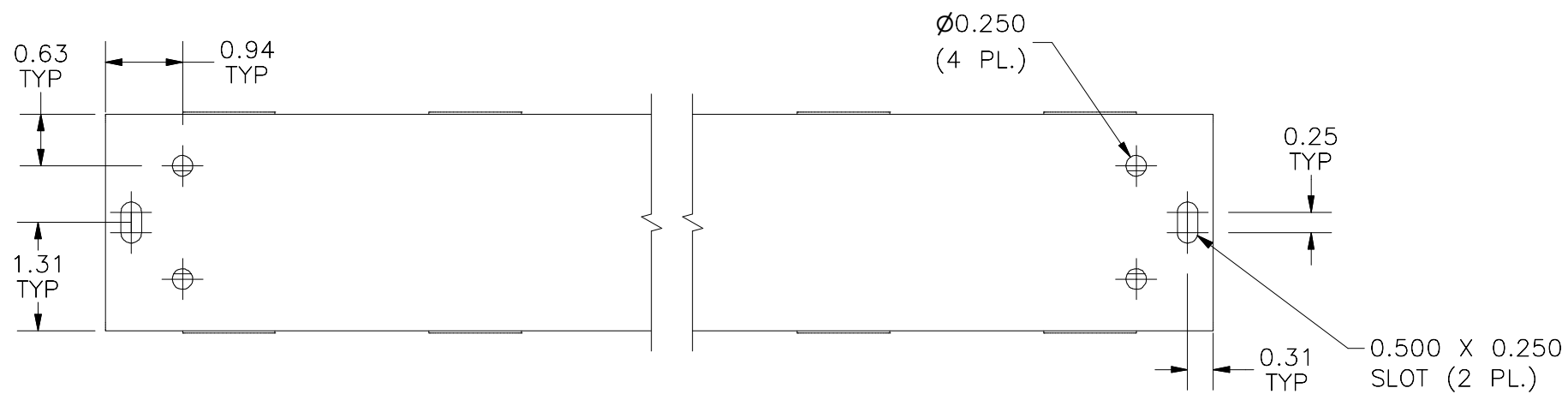
BOTTOM VIEW
