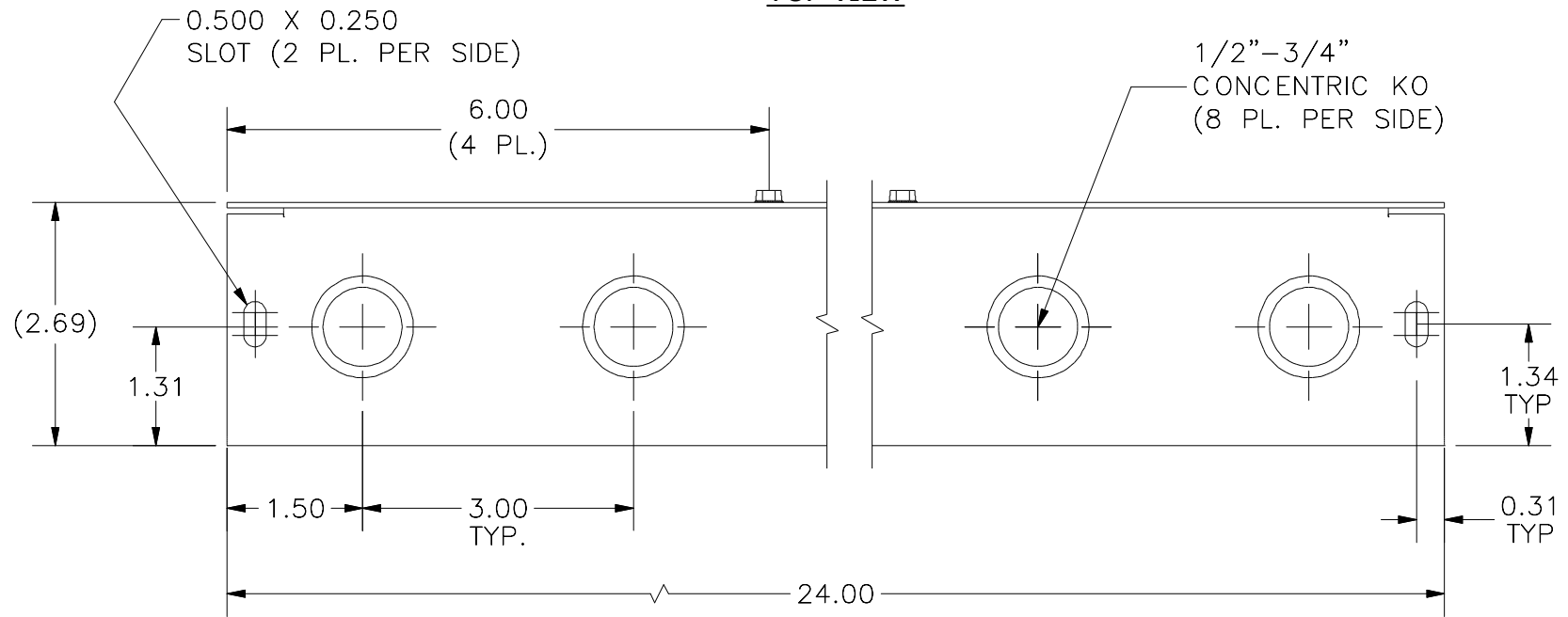
FRONT VIEW
