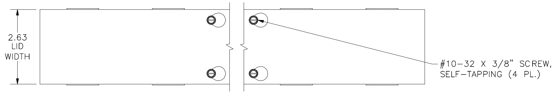
TOP VIEW
