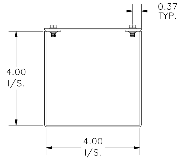
RIGHT VIEW
