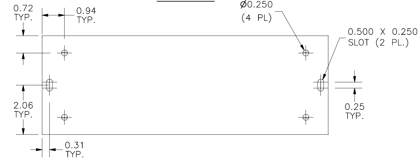
BOTTOM VIEW
