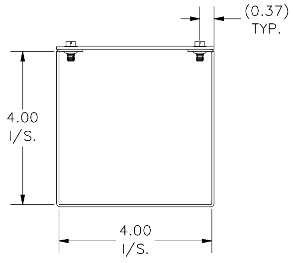
RIGHT VIEW
