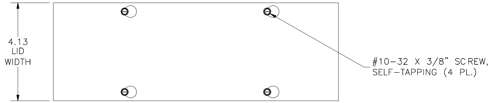
TOP VIEW
