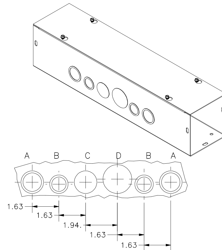
DETAIL A PATTERN DESCRIPTION (2 PL.)
