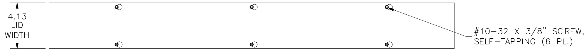
TOP VIEW
