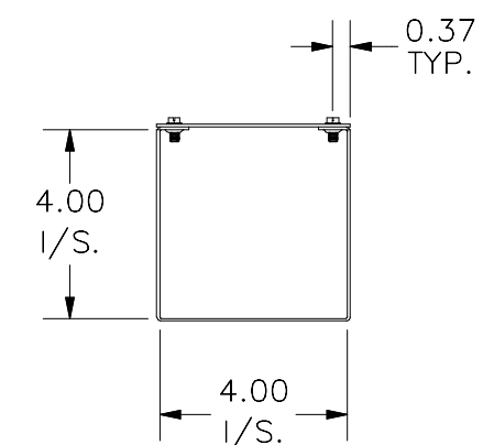
RIGHT VIEW
