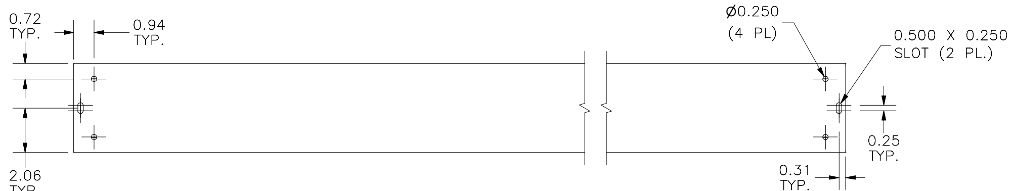
BOTTOM VIEW
