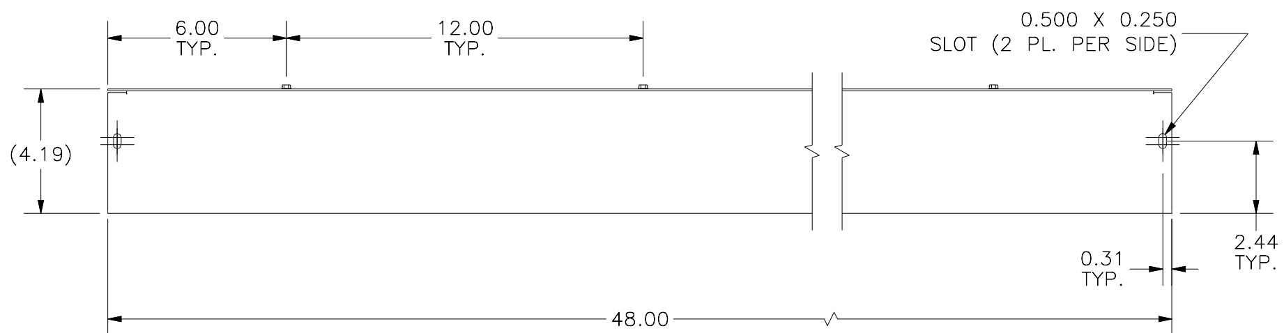
FRONT VIEW
