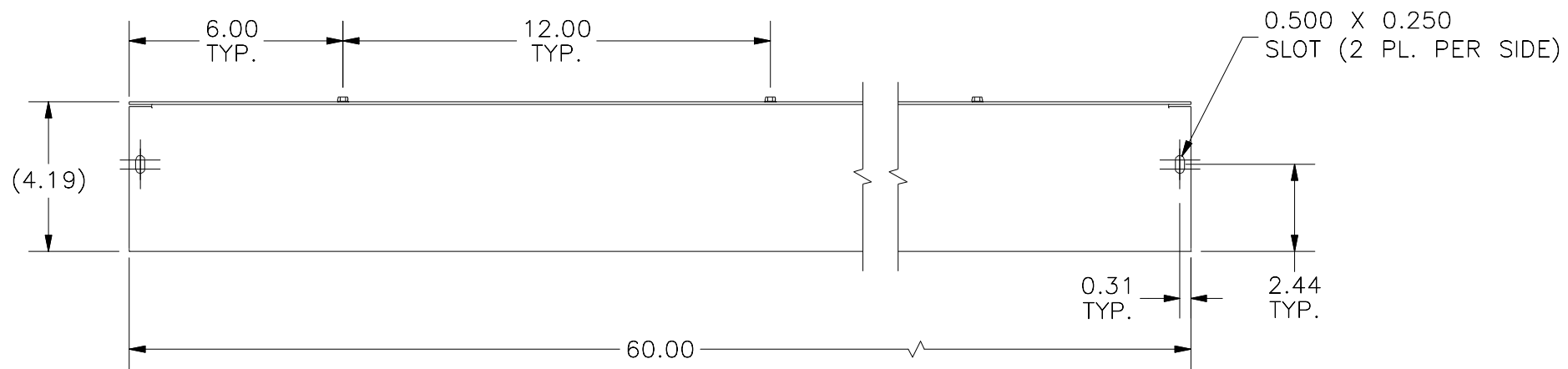
FRONT VIEW
