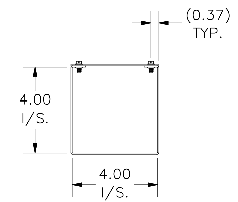
RIGHT VIEW
