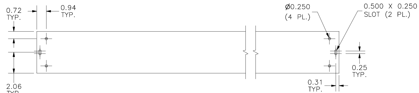
BOTTOM VIEW
