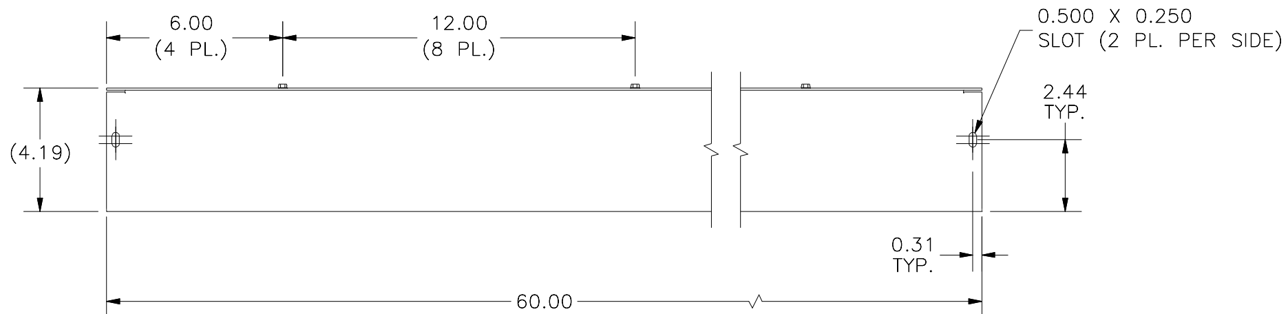
FRONT VIEW
