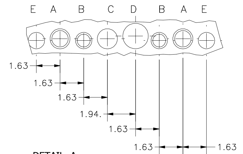
DETAIL A PATTERN DESCRIPTION (8 PL.)
