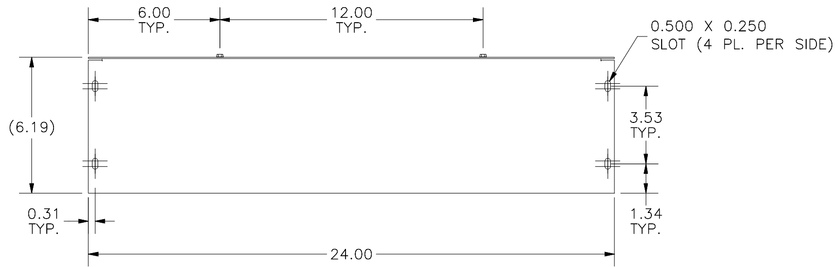
FRONT VIEW
