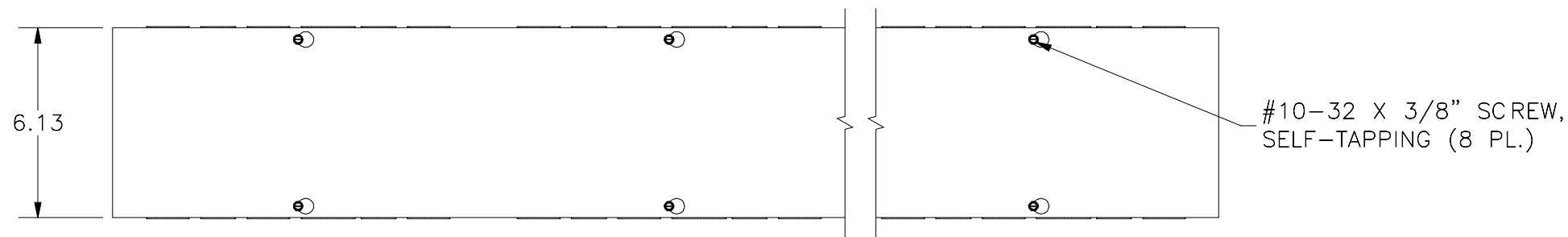
TOP VIEW
