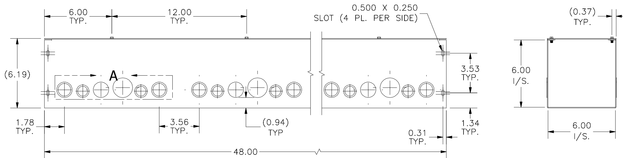
RIGHT VIEW
