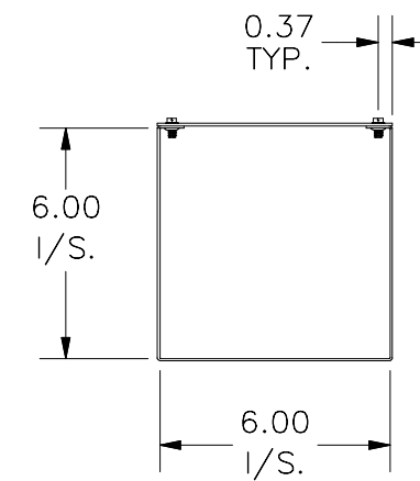
RIGHT VIEW
