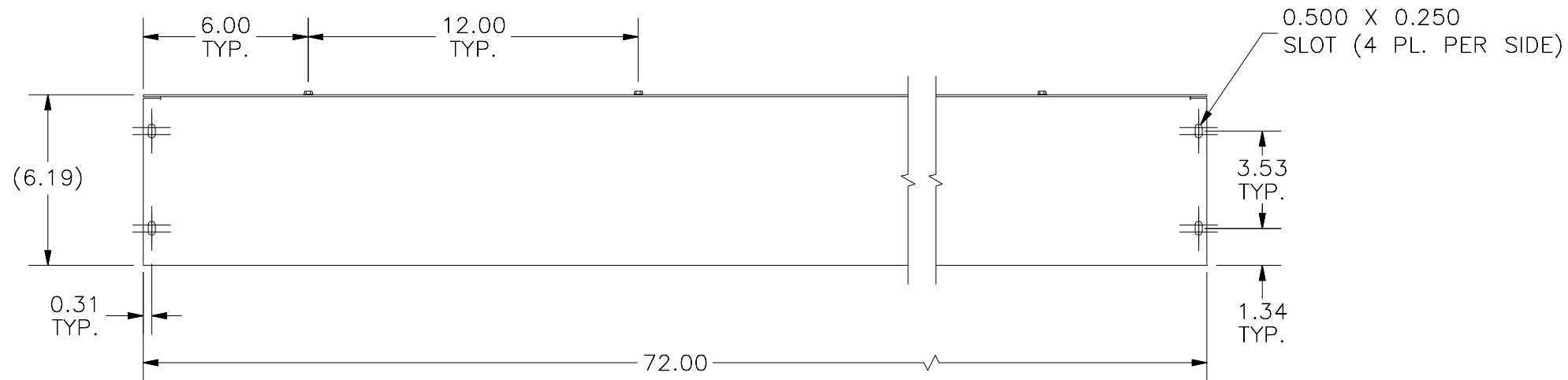
FRONT VIEW
