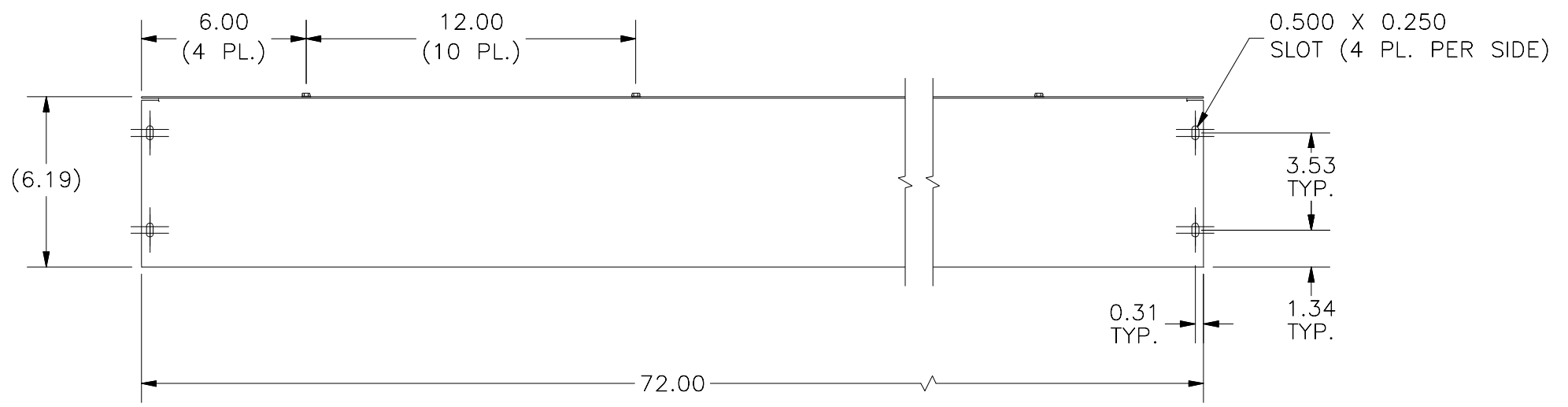
FRONT VIEW
