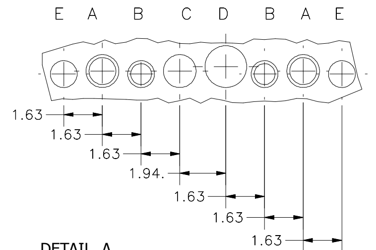
DETAIL A PATTERN DESCRIPTION (4 PL.)
