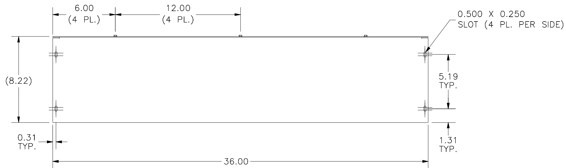
FRONT VIEW
