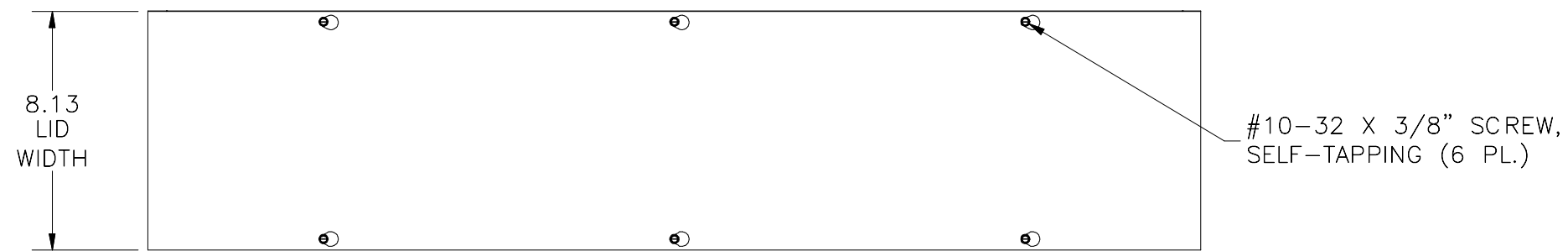
TOP VIEW
