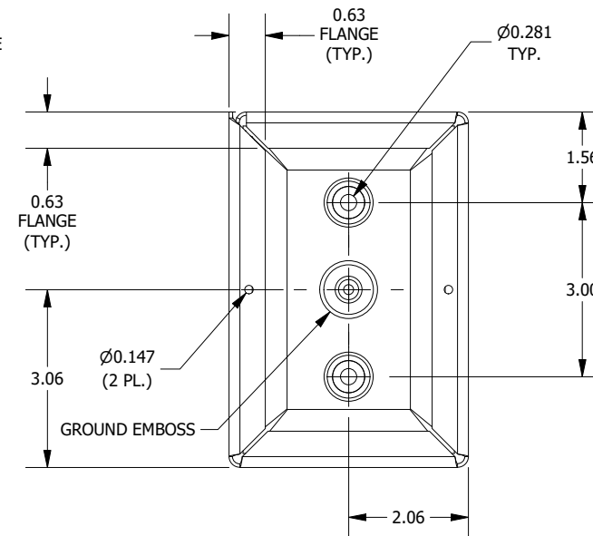
FRONT VIEW LID REMOVED
