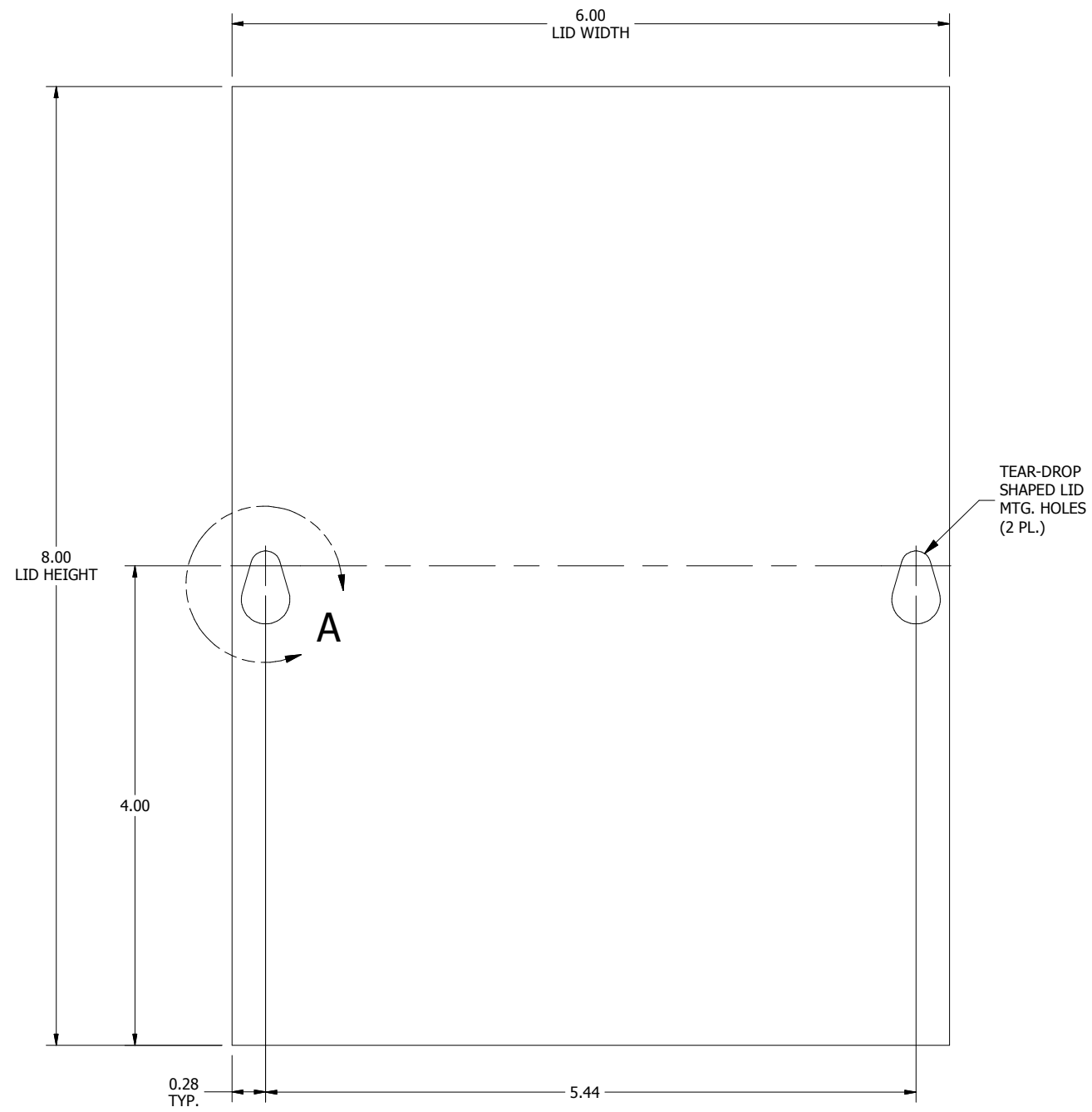
FRONT VIEW
