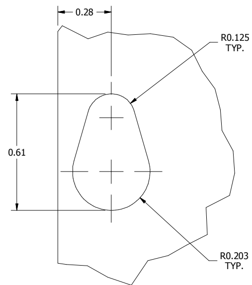
DETAIL A (MTG HOLES DETAIL VIEW)
