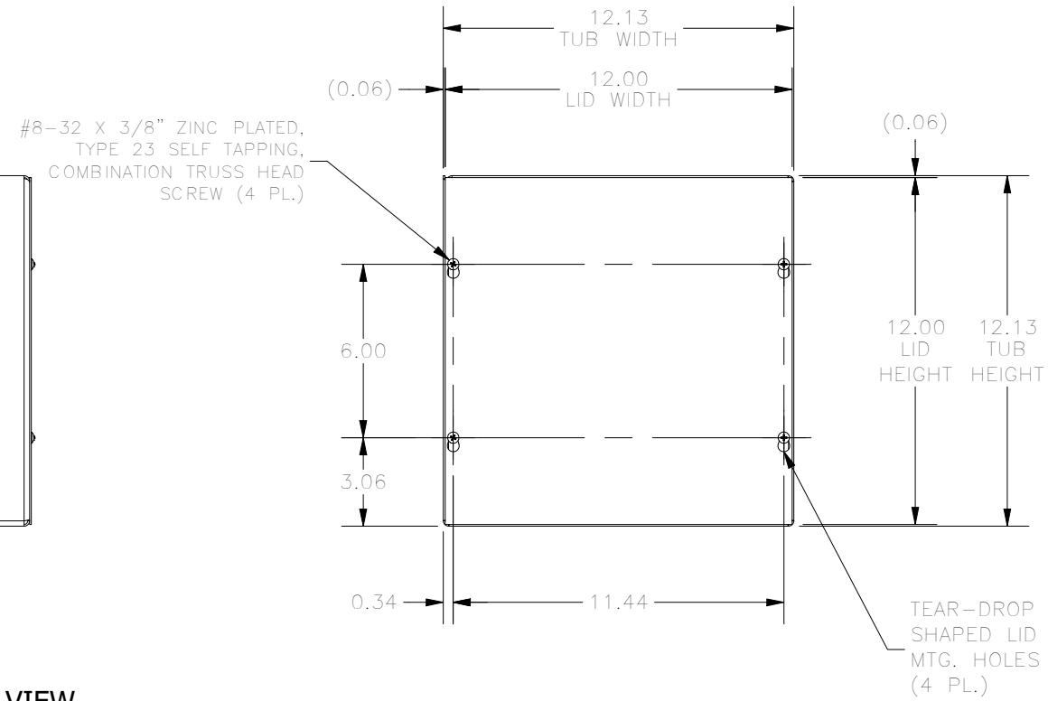
FRONT VIEW
