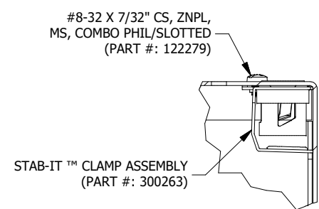
DETAIL A (6 PL.) (STAB-IT™ INSTALLATION DETAIL)
