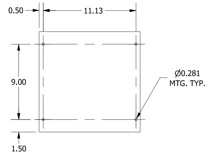
BACK VIEW
