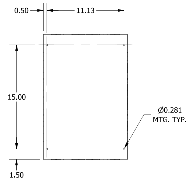
BACK VIEW
