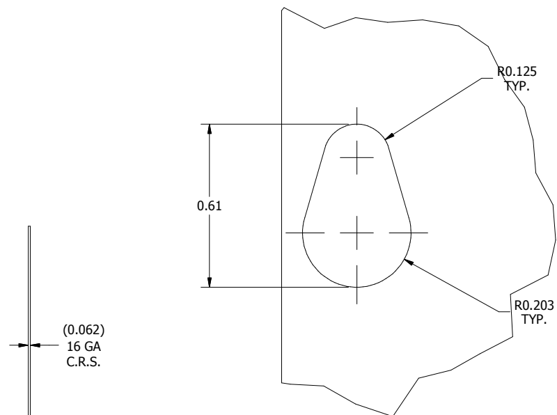
DETAIL A (MTG HOLES DETAIL VIEW)
