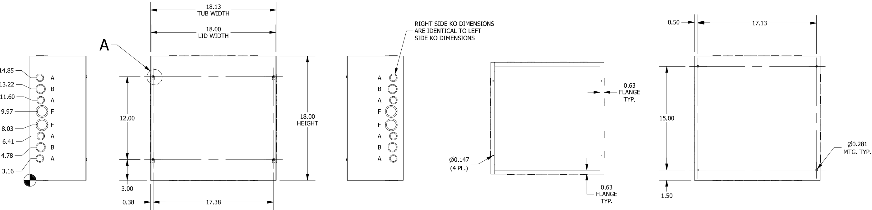
BACK VIEW
