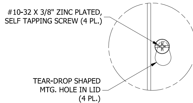
DETAIL A
