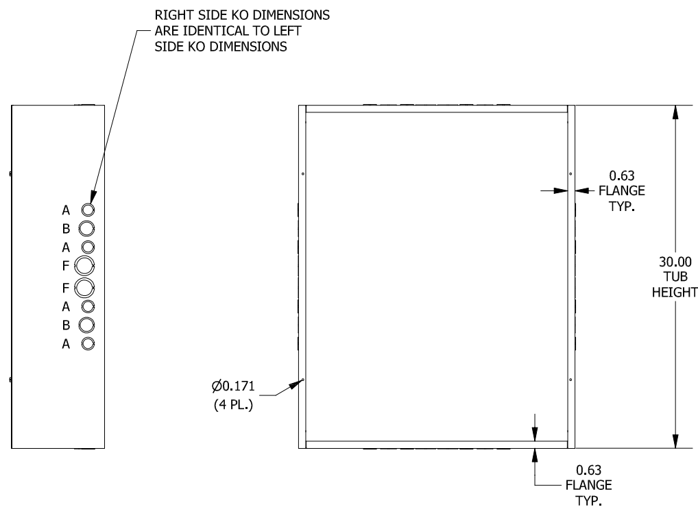
FRONT VIEW LID REMOVED
