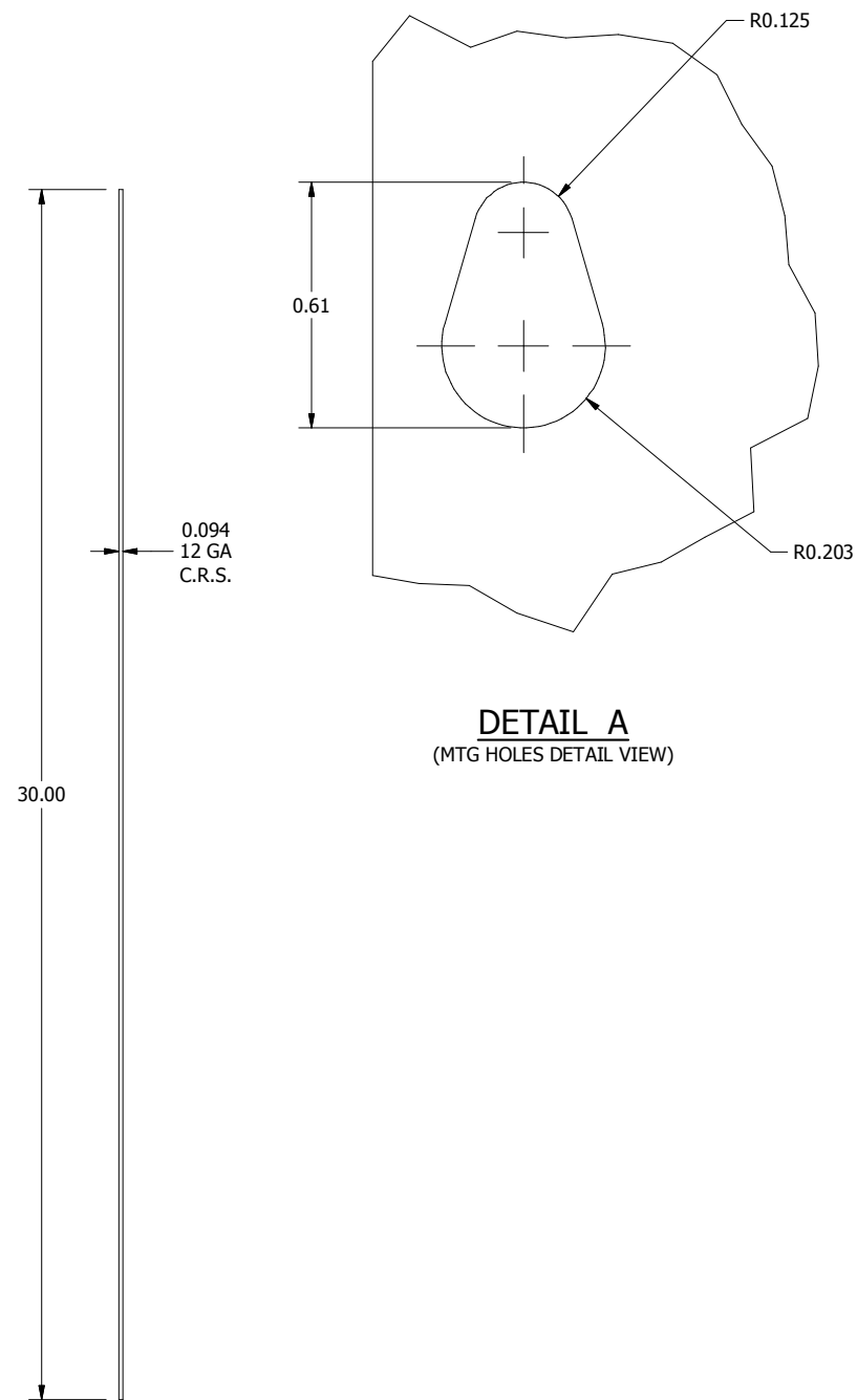
SIDE VIEW
