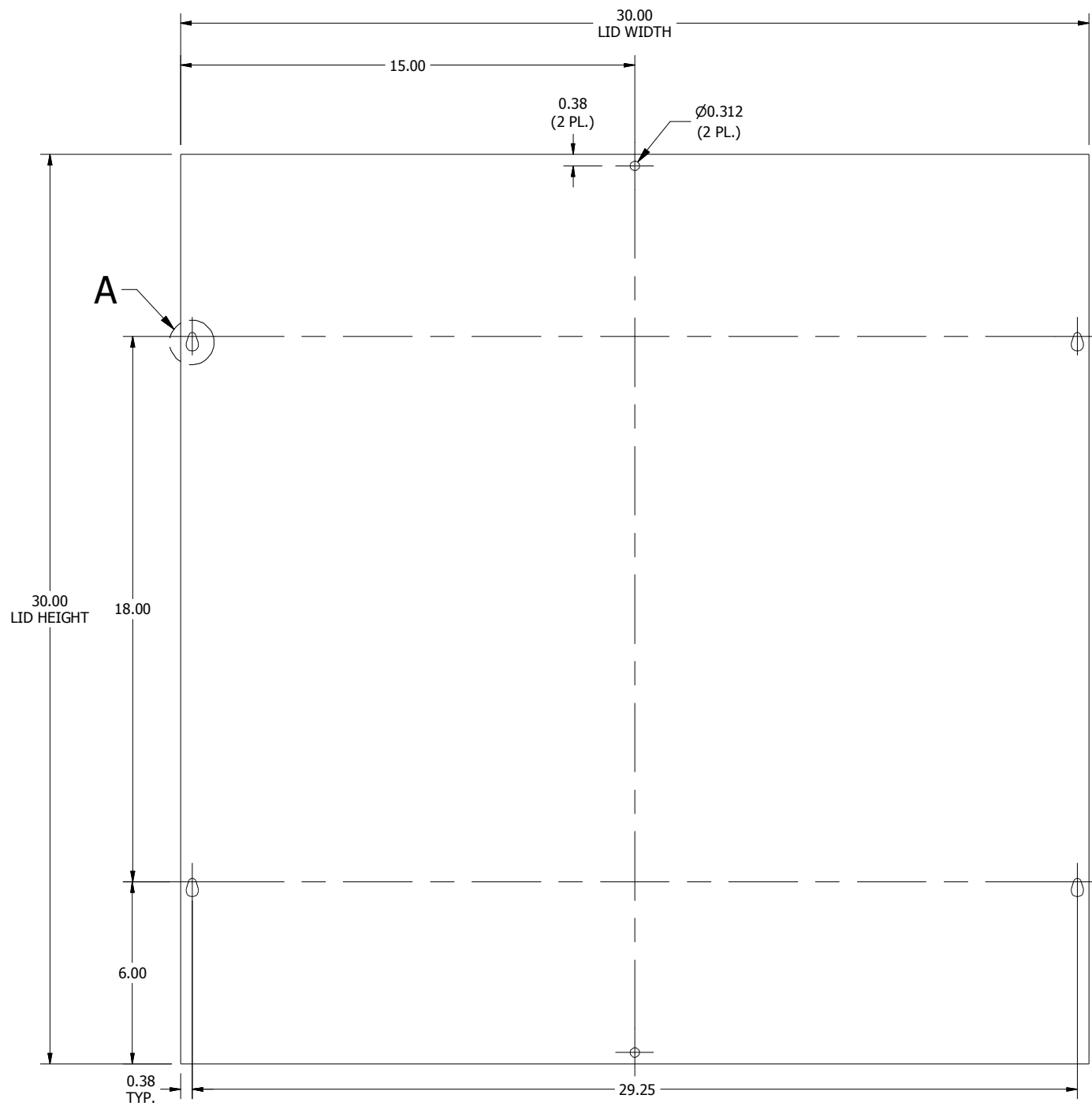
FRONT VIEW
