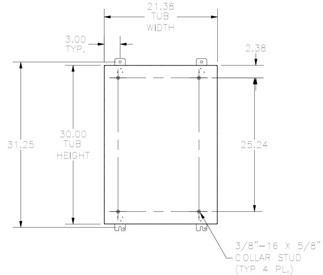
SECTION B-B (INSIDE BACK OF ENCLOSURE)
