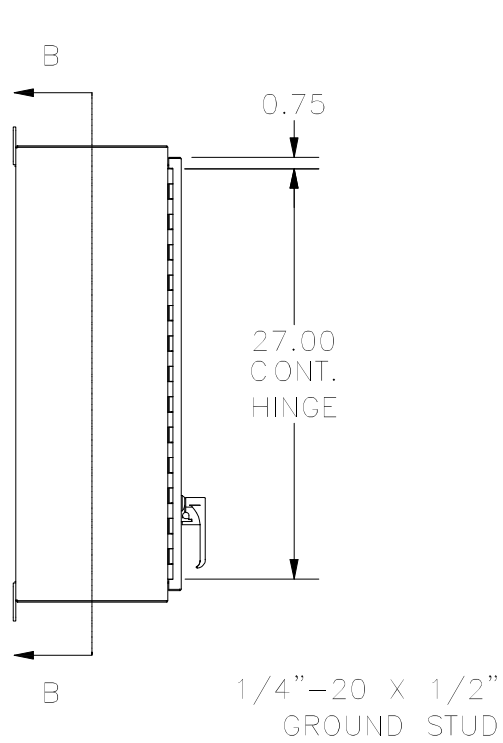
LEFT VIEW
