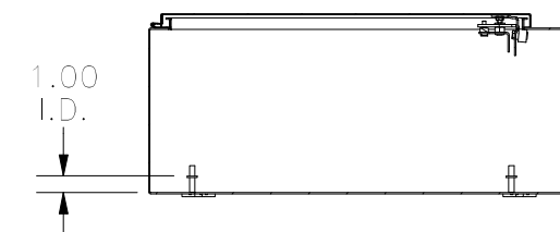
SECTION A-A (INSIDE TOP OF ENCLOSURE)
