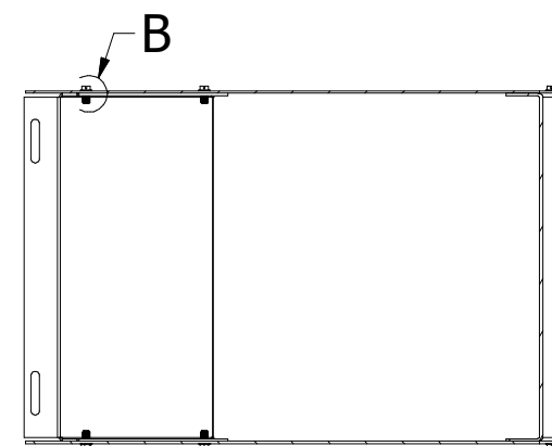
SECTION A-A (INSIDE VIEW OF SIDE)
