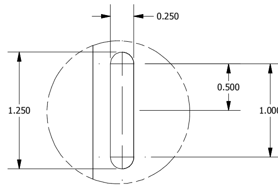
DETAIL A (22 PL.) (SLOT DETAIL)
