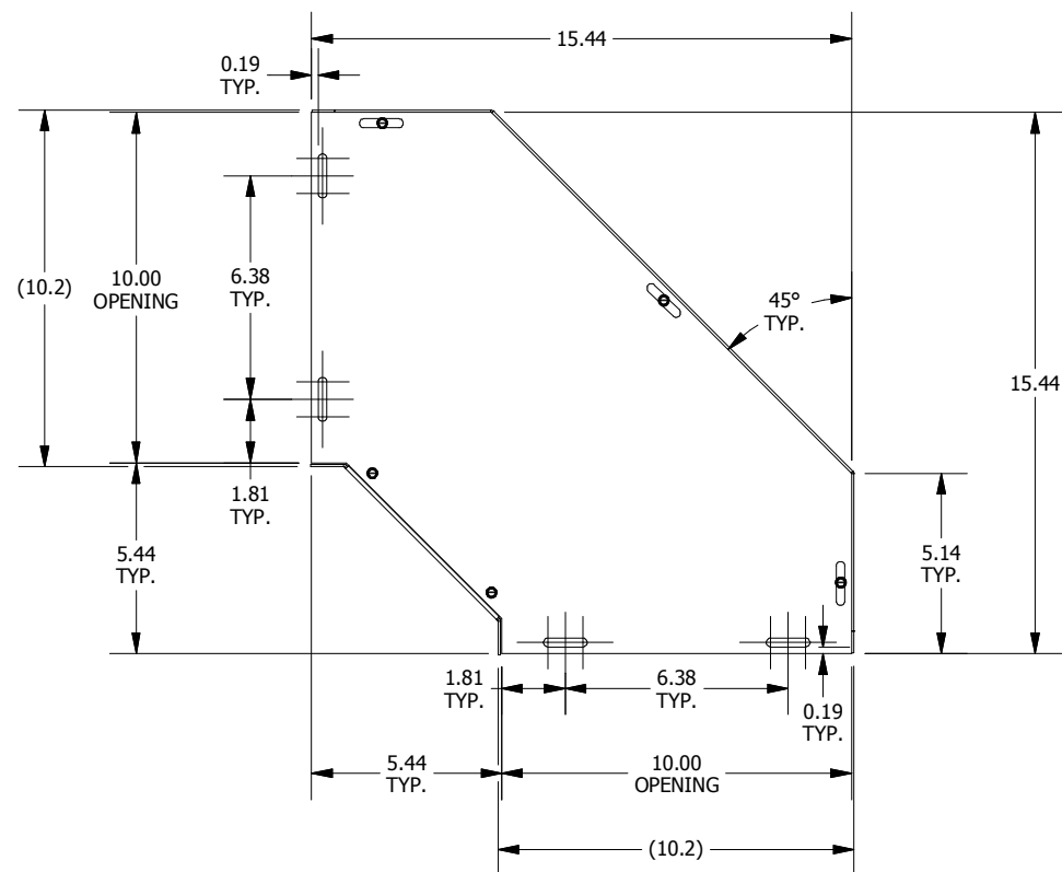
TOP VIEW
