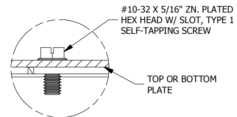
DETAIL B (10 PL.) (ASSM. DETAIL)
