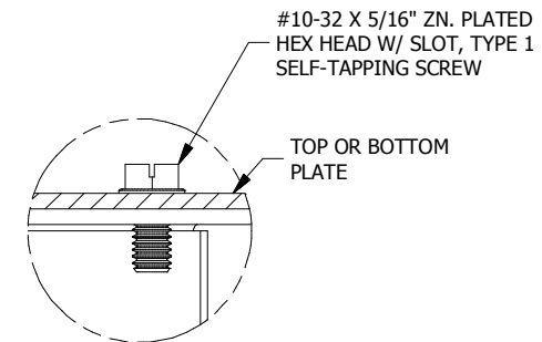
DETAIL B (10 PL.) (ASSM. DETAIL)
