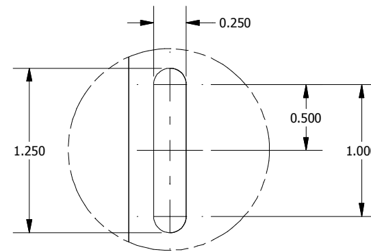
DETAIL A (26 PL.) (SLOT DETAIL)
