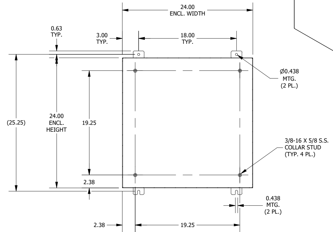
SECTION A-A (INSIDE BACK OF ENCLOSURE)
