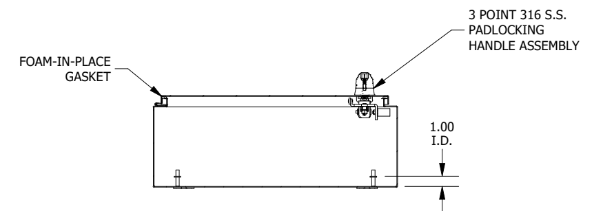
SECTION B-B (INSIDE TOP OF ENCLOSURE)
