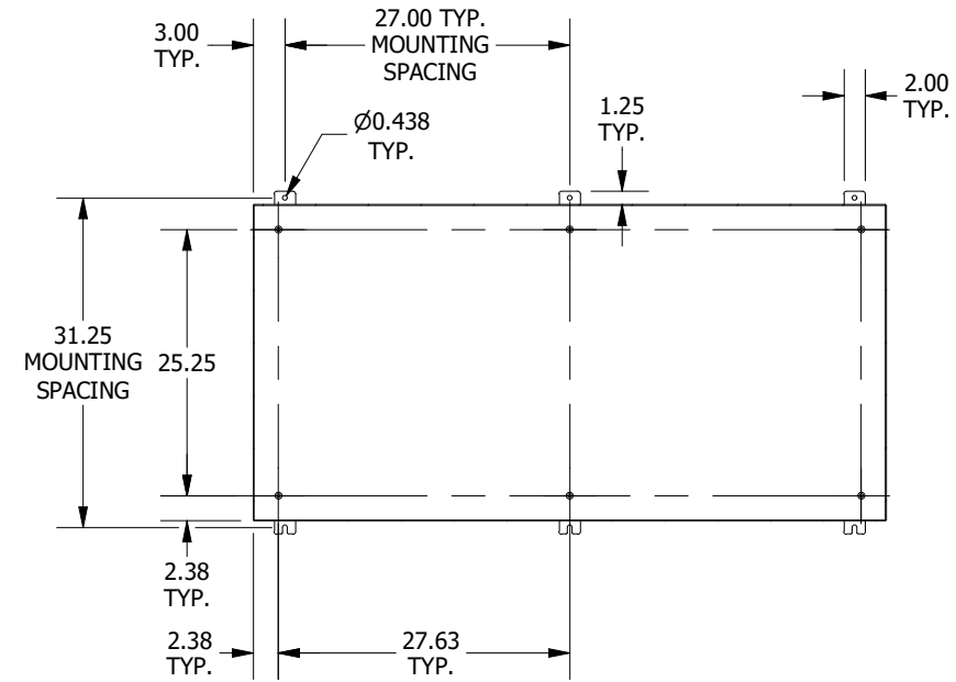
SECTION A-A (INSIDE BACK VIEW OF ENCL.)
