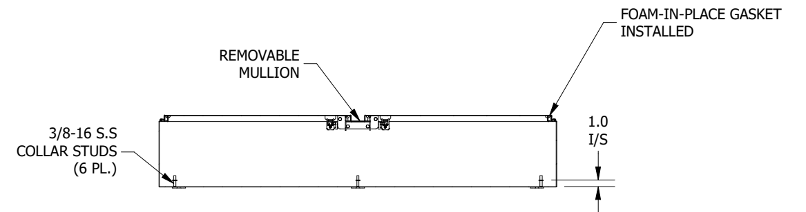
SECTION B-B (INSIDE VIEW OF TOP)
