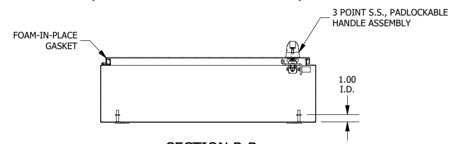
SECTION B-B (INSIDE TOP OF ENCLOSURE)
