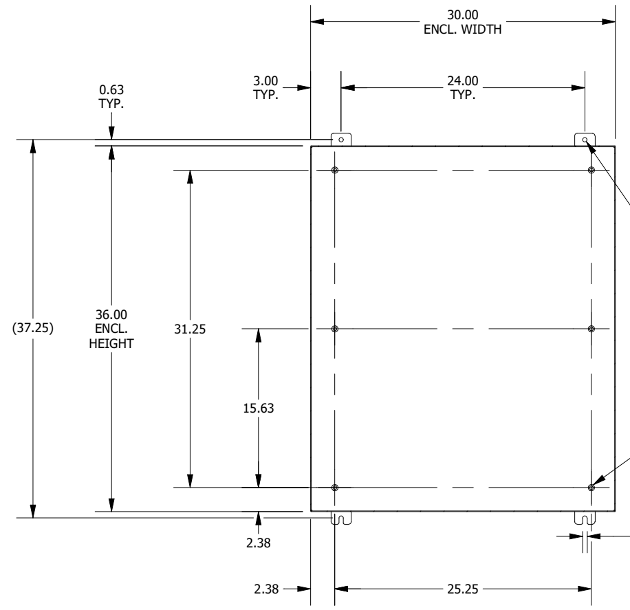
SECTION A-A (INSIDE BACK OF ENCLOSURE)
