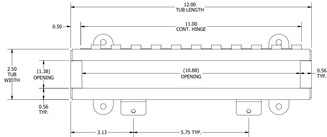
TOP VIEW (LID REMOVED)
