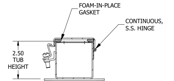
SECTION A-A (INSIDE LEFT OF ENCL.)
