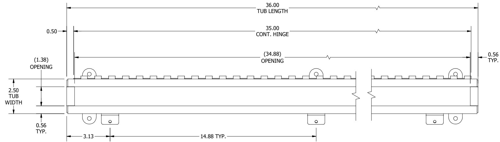
TOP VIEW (LID REMOVED)
