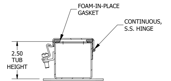
SECTION A-A (INSIDE LEFT OF ENCL.)
