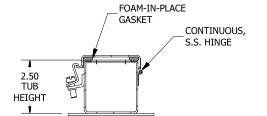
SECTION A-A (INSIDE LEFT OF ENCL.)
