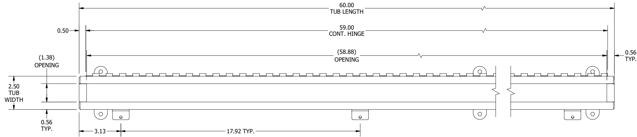
TOP VIEW (LID REMOVED)
