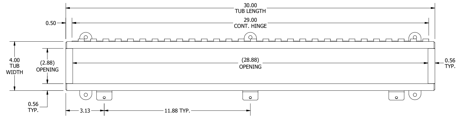
TOP VIEW (LID REMOVED)
