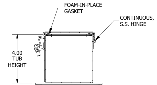
SECTION A-A (INSIDE LEFT OF ENCL.)
