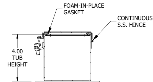
SECTION A-A (INSIDE LEFT OF ENCL.)
