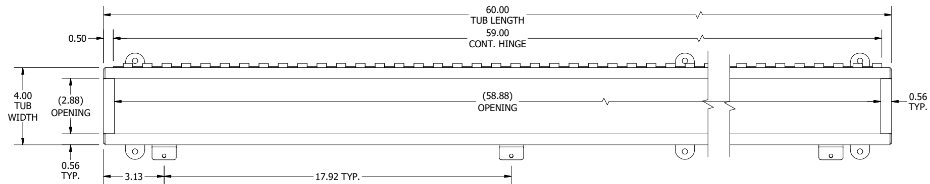
TOP VIEW (LID REMOVED)
