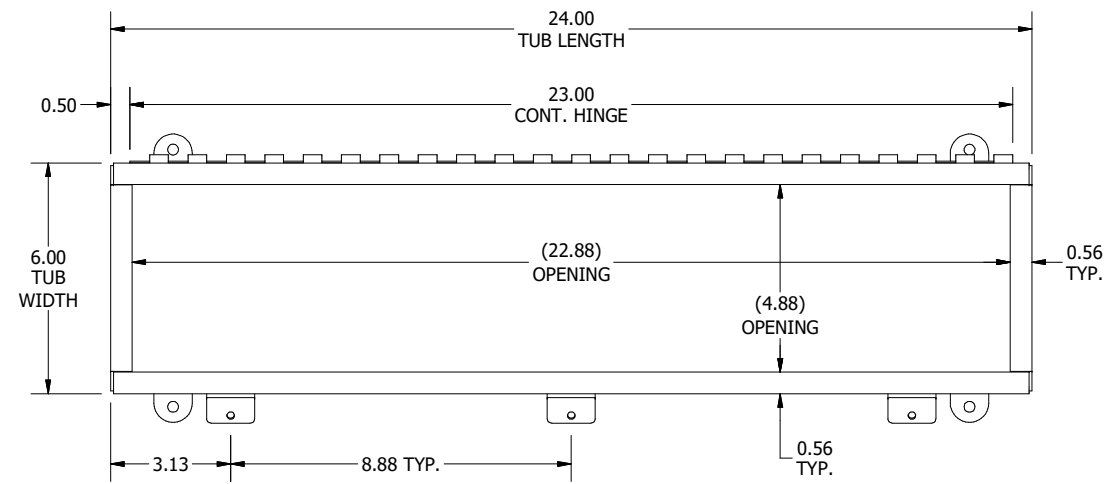
TOP VIEW (LID REMOVED)
