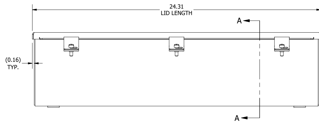
FRONT VIEW
